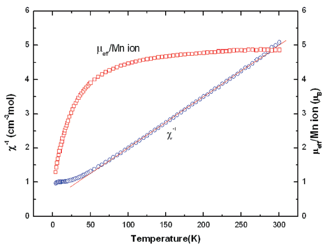
Figure 3. Temperature dependence of the effective magnetic moment per Mn ion ( \mu_{\text{eff}} ), the inverse magnetic susceptibility ( \chi^{-1} ), and its best fit (red solid line) for 2 .
