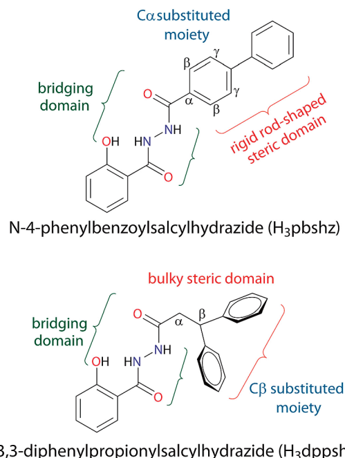
Scheme 1. A Schematic Diagram of the H 3 pbshz and H 3 dppshz Ligands
