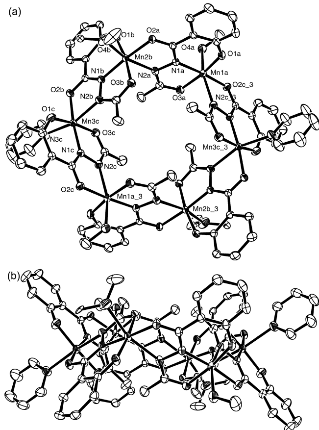
Figure 3. (a) An ORTEP drawing of complex 3 , \text{Mn}_6(\text{ashz})_6-(\text{MeOH})_4(\text{py})_2 . The complex is in the crystallographic inversion center. A, B, and C in manganese ions could be related to each other using a pseudo- S_6 symmetry operation. The methanol is coordinated to the manganese A center and B center, the pyridine is coordinated to the manganese C center. Hydrogen atoms have been omitted for clarity. (b) Side view of complex of complex 3 shows the thickness of the disc-shaped metallamacrocycle.
