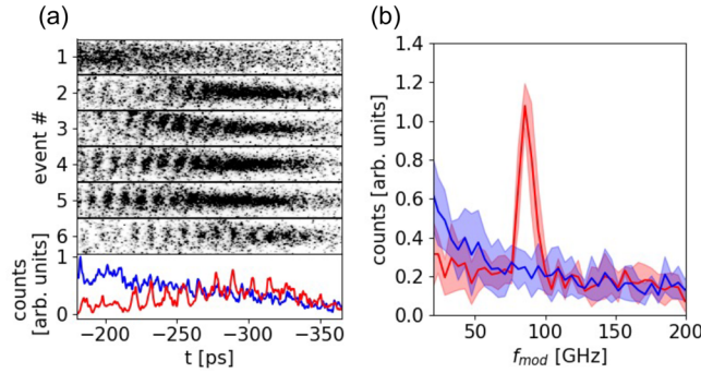
FIG. 4. (a) Six time-resolved, consecutive, single-event images of the narrow p^+ bunch. Event #1: without plasma; events #2–6: with plasma. Blue line: on-axis profile of event #1; red line: on-axis profile of event #6. The counts are normalized with respect to the maximum projection of the image without plasma. The duration of the streak camera window is 210 ps. The width of each image is \Delta y = \pm 1.25 mm centered on the beam propagation axis. (b) Average power spectra obtained from the DFT of the on-axis profiles of single-event images. Red line: average of the power spectra of five consecutive events with plasma [events #2–6 from (a)]; blue line: average of the power spectra of five consecutive events without plasma (including event #1). The shaded areas show the extent of the rms variations. Same color scale for all images. n_{pe} = 0.97 \times 10^{14} \text{ cm}^{-3} , f_{pe} = 88.3 \text{ GHz} .
