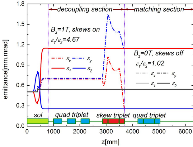
Figure 2: Evolution of the rms emittances and eigen-emittances along the EMTEX beam lines for two cases.
