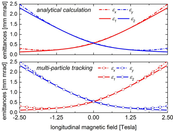
Figure 3: Eigen-emittances and rms emittances calculated by analytical method based on the decoupling matrix of Equ. (23) and by multi-particle tracking through the EMTEX beam line.
