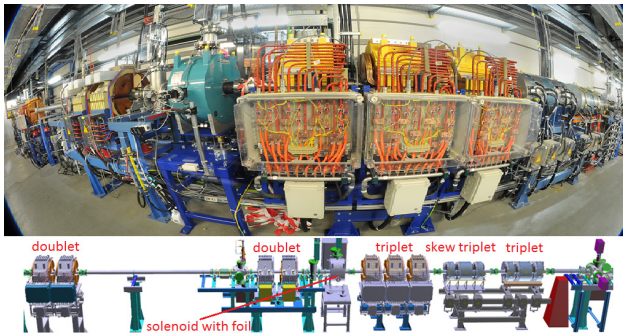
Figure 1: Emittance transfer experiment (EMTEX) beam line for demonstration of transverse rms emittance transfer.
