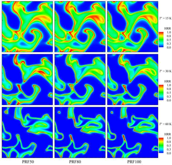
Fig. 2 Isocontours of normalized HRR (from left to right, PRF50, PRF80 and PRF 100 at t/\tau_{ig} = 0.88, 0.91, and 0.95 with T' = 15 K (top); t/\tau_{ig} = 0.79, 0.80, and 0.82 with T' = 30 K (middle); t/\tau_{ig} = 0.62, 0.59, and 0.59 with T' = 60 K (bottom).
